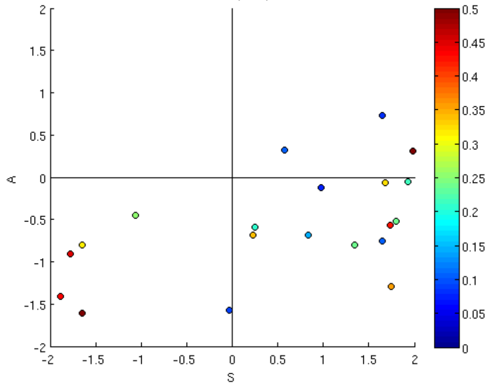
AROME 20080901-20080930 18UTC, 3h acc precip +09 and +15, #OB<20, sumOB<4000
