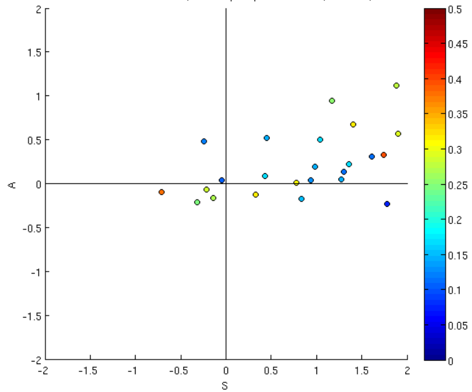
ALARO 20080901-20080930 18UTC, 3h acc precip +09 and +15, #OB<20, sumOB<4000
