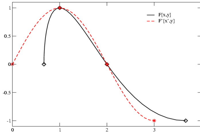
Fig.1: The true function F to be interpolated on stretched model grid fitting the model gridpoints (black full line with the points marked as diamonds) and the equivalent function F' transformed to regular grid which is interpolated instead along vertical during spline interpolation (red dashed curve with the points marked as stars). The target area to be interpolated is located between points 1 and 2 on x-axis.
