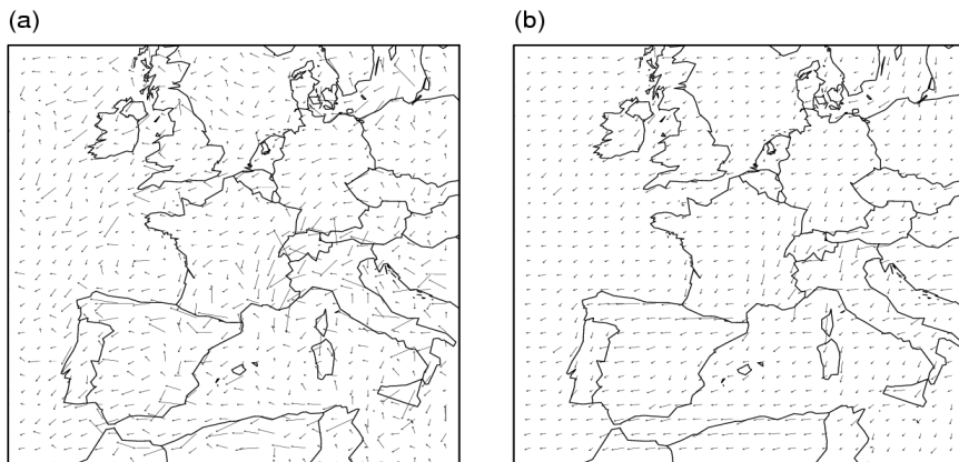
Local anisotropy axes at model level 41 (a) from raw data and (b) from Bw
