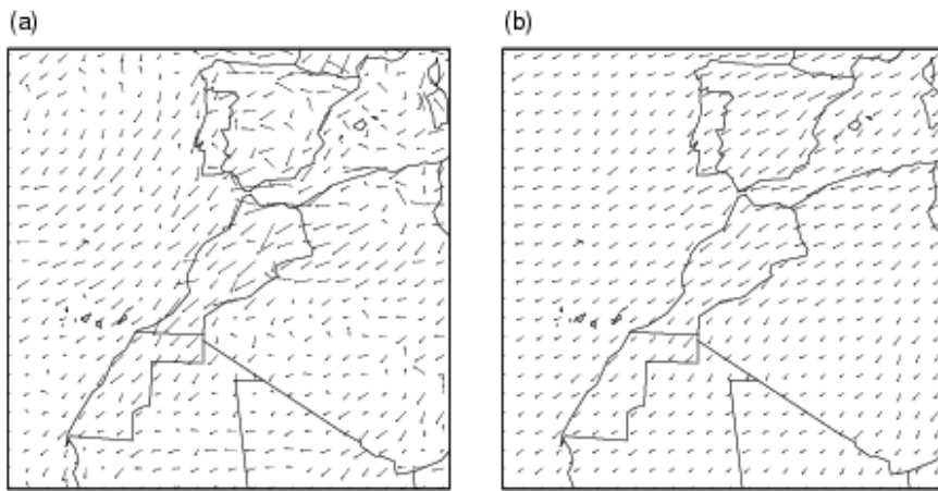
Local anisotropy axes at model level 31: (a) from raw data and (b) from Bw
