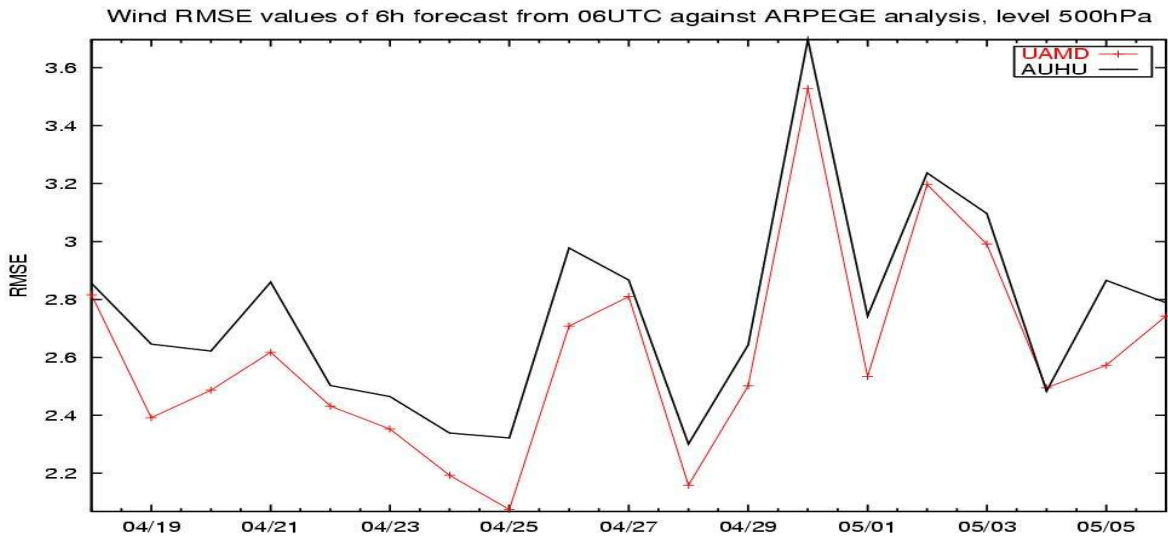
Figure 8.: Root-mean-square error (m/s) of 6-hour forecast from 06 UTC of wind field observed every day. Legend as in Fig. 7.
