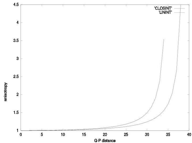
Fig. 3 : Degree of anisotropy for the two formulations : CLOSINT, nearest-integer estimation (5) and LININT, linear interpolation (6)
