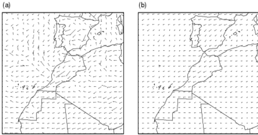
Local anisotropy axes at model level 13; (a) from raw data and (b) from Bw
