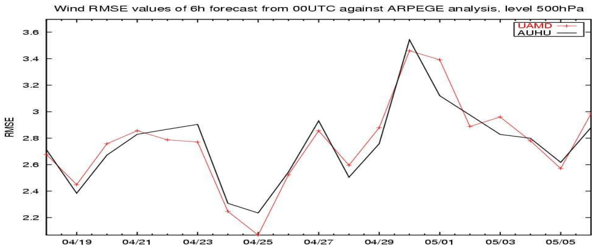
Figure 10.: Root-mean-square error of 6-hour forecast from 00 UTC of wind field observed every day. Legend as in Fig. 8.
