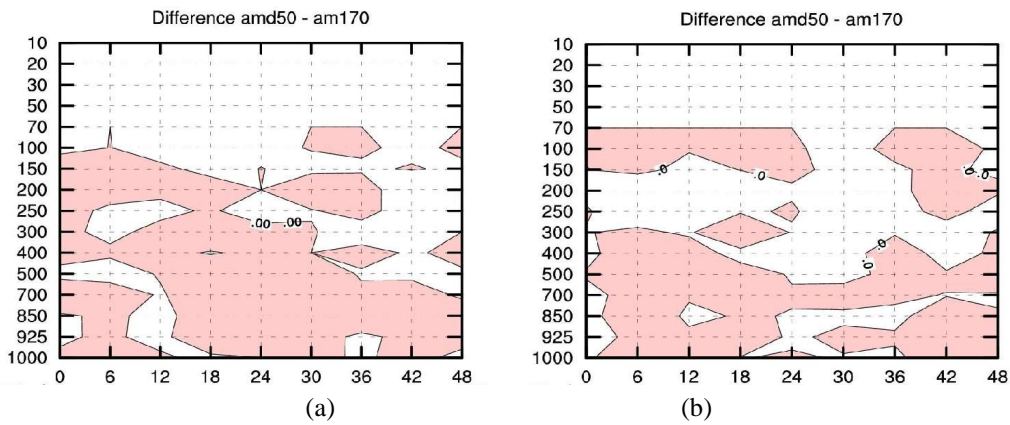
Figure 4.: Difference between the root-mean-square errors (RMSE) for temperature (a) and wind speed (b) : RMSE_{amd50} - RMSE_{amd170} .
