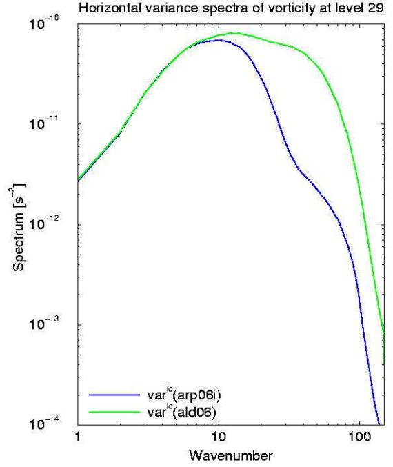
Figure 2: Dispersion spectra related to the initial condition perturbations for initialized ARPEGE first guess and ALADIN background fields
