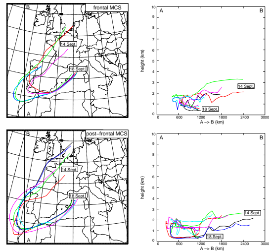
Fig. 18. Backward trajectories of some air parcels taken in the moist low-level flow feeding the 18 September 2009 precipitating systems obtained with the RA110 simulation in two different phases of the event – convection embedded in a frontal disturbance (top) and post-frontal mature convection (bottom). The backward trajectories are projected both on an horizontal plane (left panels) and on a vertical cross-section (right panels). The vertical cross-section follows the line AB displayed on the left panels.
