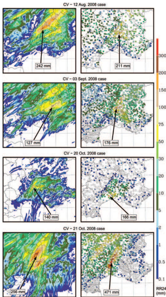
Fig. 3. 24-h accumulated precipitation ( \pi_{24} in mm) from the HRA2.5 simulations (left panels) and the Météo-France rain-gauge network (right panels) at 00:00 UTC, 13 August 2008 for the 12 August 2008 case (top), at 06:00 UTC, 4 September 2008 for the 3 September 2008 case (middle top), at 00:00 UTC, 21 October 2008 for the 20 October 2008 case (middle bottom) and at 06:00 UTC, 22 October 2008 for the 21 October 2008 case (bottom). The maximum of precipitation is indicated on each panel.
