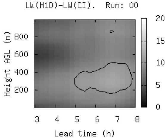
Figure 4.- Average difference between the outgoing long-wave radiation forecast by H1D and COBEL-ISBA in \text{Wm}^{-2} in the runs started at 00 UTC.
