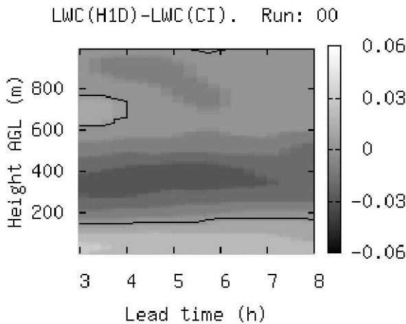
Figure 3.- Average difference between the vertical profile of liquid water forecast by H1D and COBEL-ISBA in gkg-1 in the runs started at 00 UTC.
