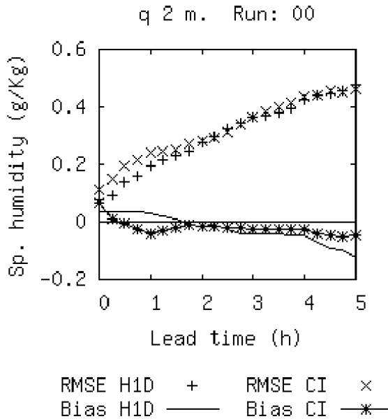
Figure 6.- Verification scores of the screen-level specific humidity forecasts issued by the 00-runs of H1D and COBEL-ISBA.
