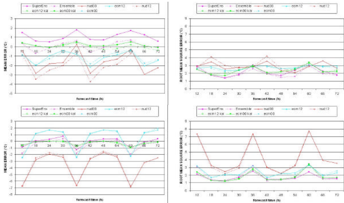
Figure 2: Temperature results for Torino venue (top) and Sestriere venue (bottom). Left column: mean error with respect to observations. Right column: root mean square error. Pink lines: Multimodel Ensemble and SuperEnsemble results; blue lines: ECMWF direct model output; green lines: Kalman filter calculated from ECMWF; red lines: COSMO- LAMI direct model output.
