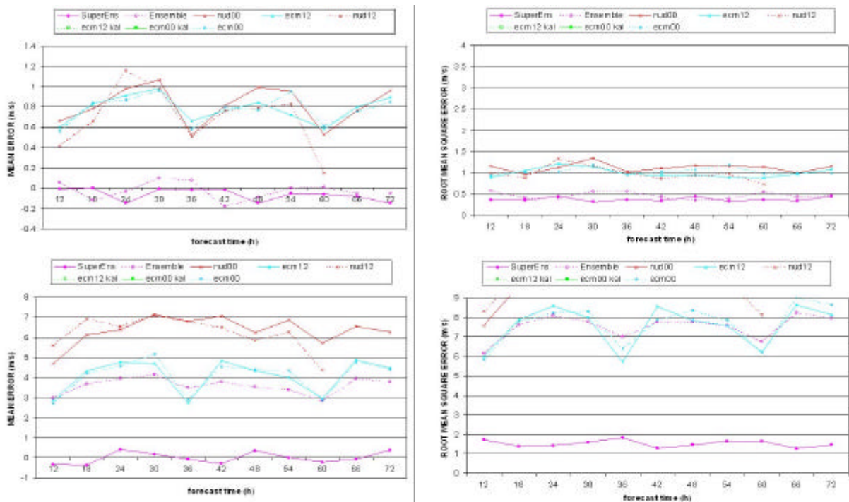
Figure 3: Wind results for Torino venue (top) and Sestriere venue (bottom). Left column: mean error with respect to observations. Right column: root mean square error. Pink lines: Multimodel Ensemble and SuperEnsemble results; blue lines: ECMWF direct model output; green lines: Kalman filter calculated from ECMWF; red lines: COSMO- LAMI direct model output.
