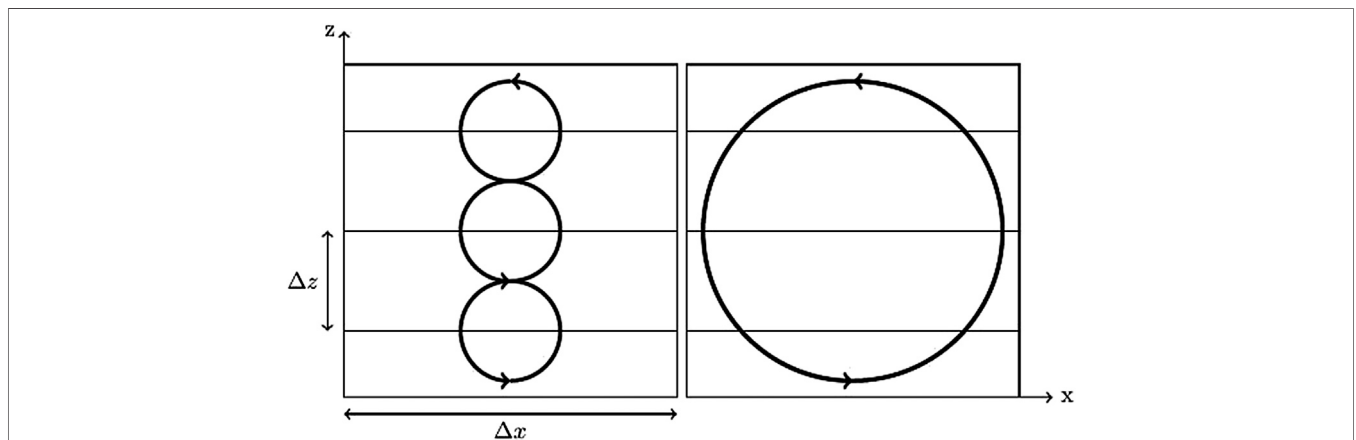
FIGURE 3 | Schematic turbulent eddy in the gray zone of turbulence when the mixing length depends on \Delta z (left) or not (right).
