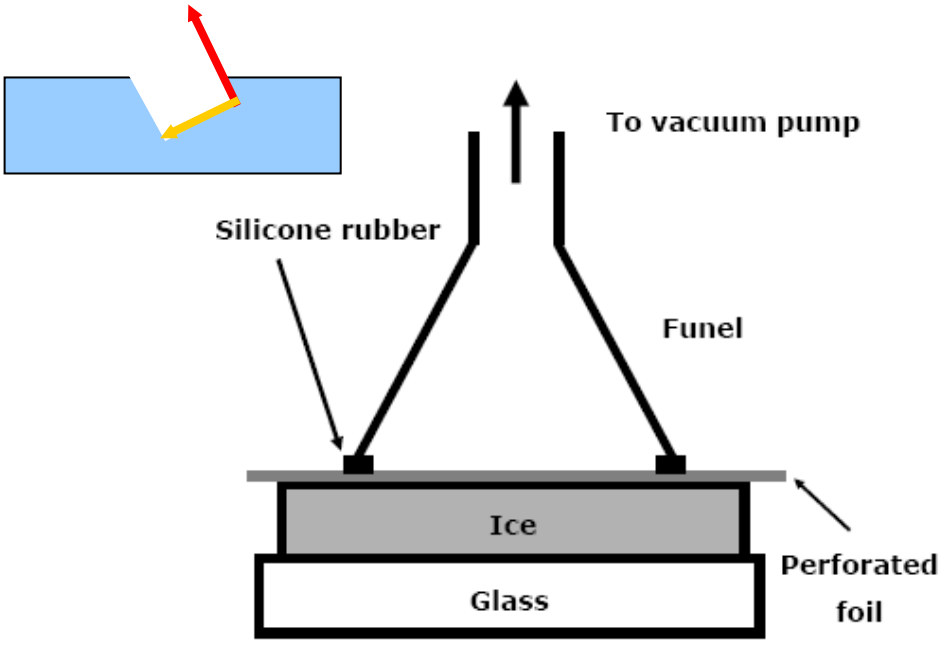
Obtaining etch pits (Knight, 1966)
